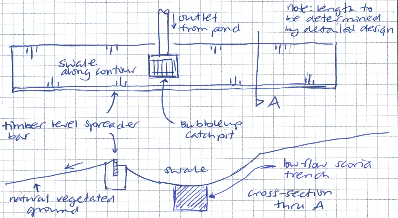
Pond outlet swale / level spreader concept
