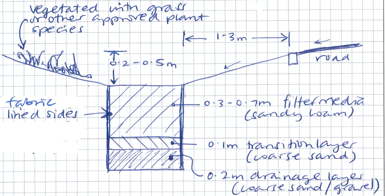
Bioretention swale (as per WRC SW guidelines Fig 8-13)
